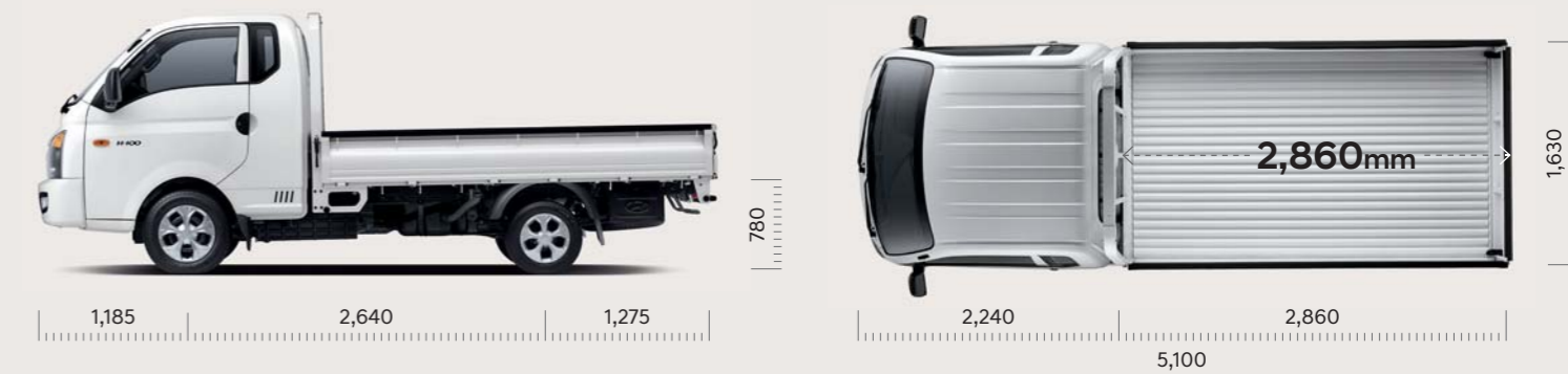
Extra long wheel base super cab (Low type rear deck)
