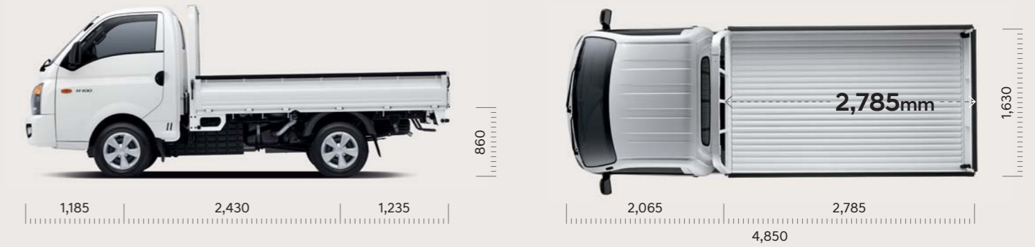
Long wheel base standard cab (High type rear deck)
